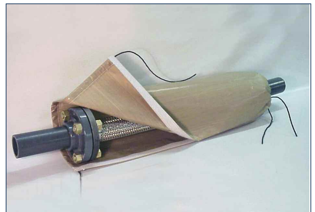
Section flexible
